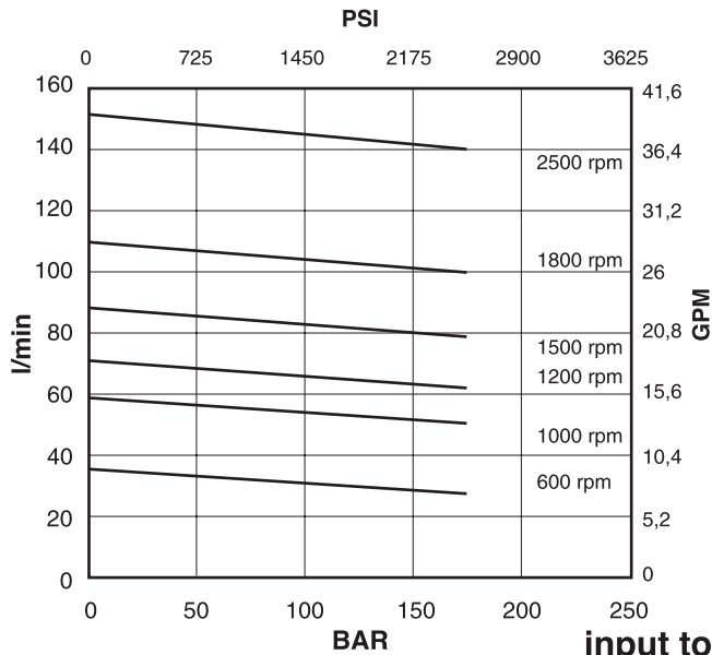
flow / pressure
